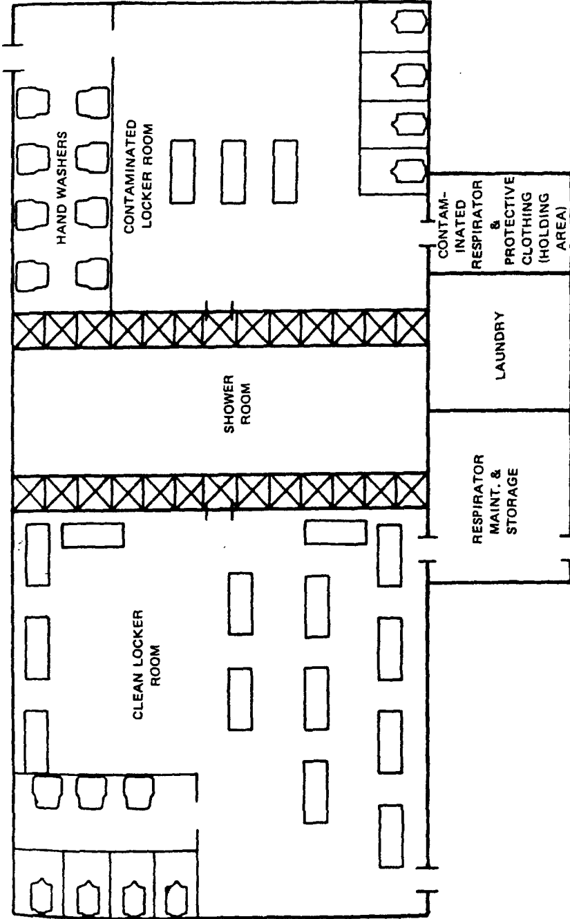
FIGURE 3 LOCKER ROOM, SHOWER ARRANGEMENT
