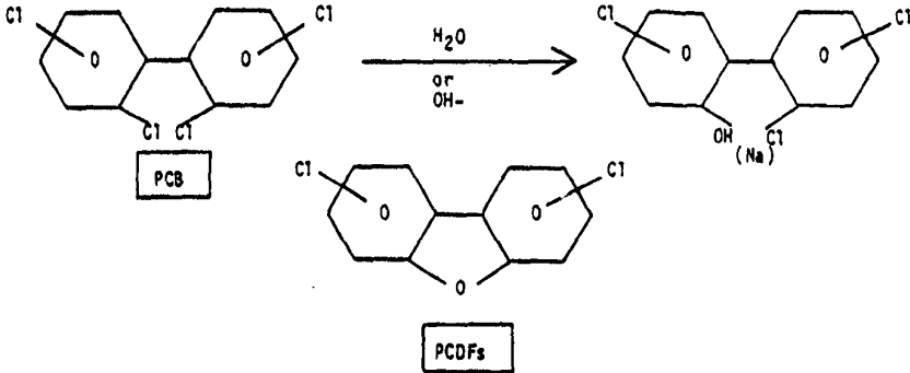
Figure 3 Conversion of PCBs to PCDFs During Purification Process
