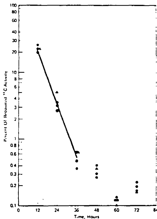
FIG. 2. 14 C-Activity excreted in the urine expressed as percentage of the recovered radioactivity versus time following a 6 hr exposure to 5000 ppm of [ 14 C]VC. Repeatedly exposed rats (▲) and singly exposed rats (●).
