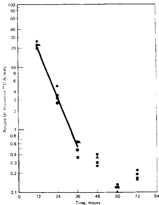
FIG. 2. ^{14}\text{C} -Activity excreted in the urine expressed as percentage of the recovered radioactivity versus time following a 6 hr exposure to 5000 ppm of ^{14}\text{C} VC. Repeatedly exposed rats (▲) and singly exposed rats (●).
