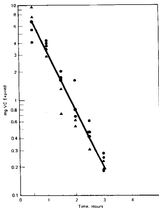
FIG. 1. Expired vinyl chloride (milligrams) versus time following a 6 hr exposure to 5000 ppm of ^{14}\text{C} VC. Repeatedly exposed rats (▲) and singly exposed rats (●).
