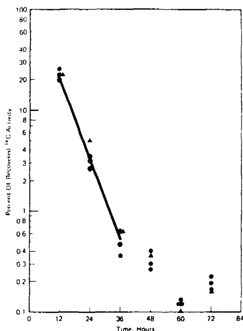
FIG. 2. ^{14}\text{C} -Activity excreted in the urine expressed as percentage of the recovered radioactivity versus time following a 6 hr exposure to 5000 ppm of ^{14}\text{C} VC. Repeatedly exposed rats ( \blacktriangle ) and singly exposed rats ( \bullet )
